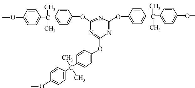
Structure motif of a polycyanurate prepared from 2,2-bis(4-cyanatophenyl)propane (bisphenol A dicyanate)
