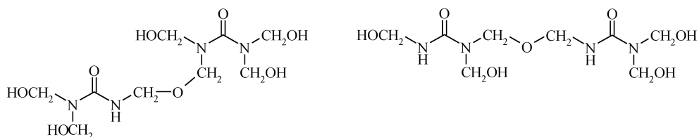
Examples of species present in a urea-formaldehyde resin
