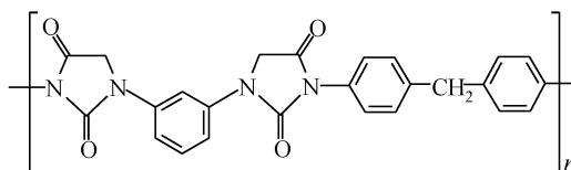
poly[(2,5-dioximidazolidine-1,3-diyl)-1,3-phenylene-(2,4-dioximidazolidine-1,3-diyl)-1,4-phenylenemethylene-1,4-phenylene]
