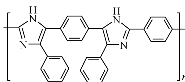
poly[(4-phenylimidazole-2,5-diyl)-1,4-phenylene-(4-phenylimidazole-5,2-diyl)-1,4-phenylene]
