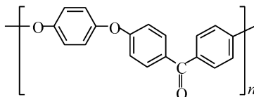
poly(oxy-1,4-phenyleneoxy-1,4-phenylene-carbonyl-1,4-phenylene)
