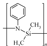
poly[(phenylimino)(dimethylsilanediyl)]
