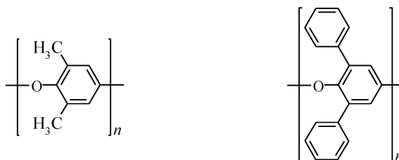
poly[oxy(2,6-dimethyl-1,4-phenylene)]
