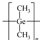
poly(dimethylgermanediyl)
