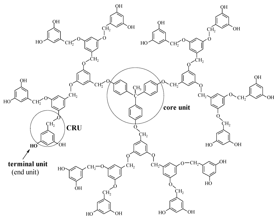
\alpha -[ethane-1,1,1-triyltri(1,4-phenylene)]- \omega -hydroxy-dendro-(oxymethylenebenzene-1,3,5-triyl) core unit terminal units constitutional repeating units (end units) (CRU)
