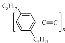
poly[(2,5-dioctyl-1,4-phenylene)ethynediyl]
