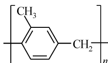
poly[(2-methyl-1,4-phenylene)methylene]
