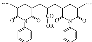
Structure motifs of a polyglutarimide prepared from poly(alkyl acrylate) and aniline
